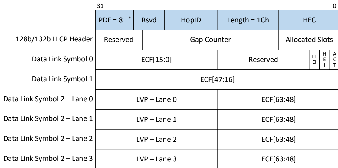
Figure 10-51. 128b/132b LLCP Packet Format
